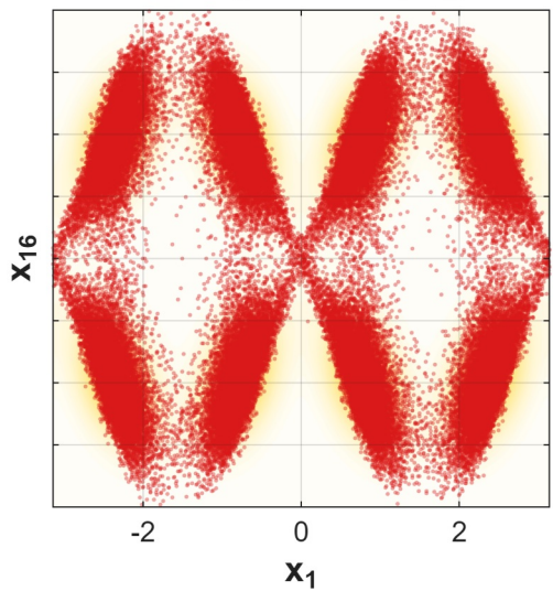
Jeffreys Flow x_1 - x_{16}
