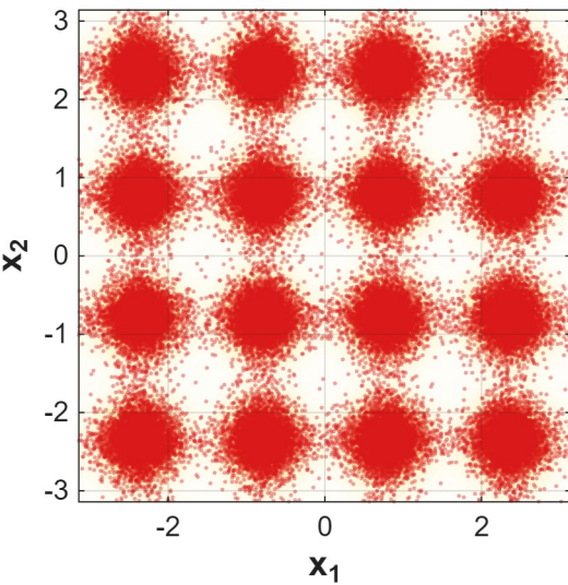
Jeffreys Flow x_1 - x_2
