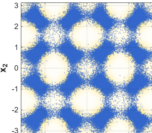
Jeffreys Flow x_1 - x_2
