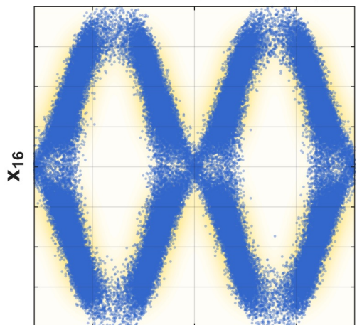
Jeffreys Flow x_1 - x_{16}
